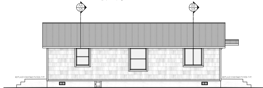
EAST ELEVATION 1/4" = 1'-0"
