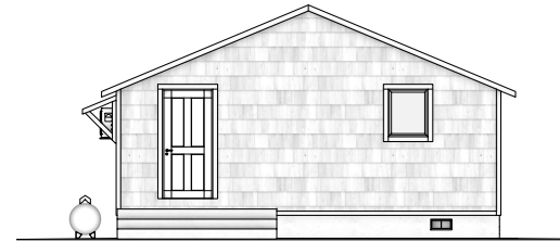
SOUTH ELEVATION 1/4" = 1'-0"
